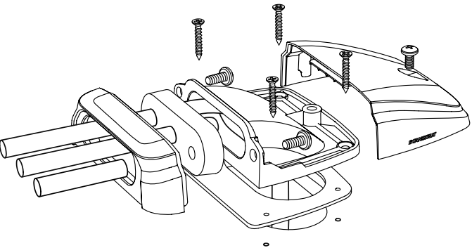
Horizontal Multi Cable Seal Designed for multiple cable installations
