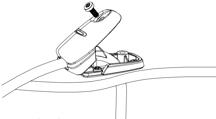
Horizontal Cable Seal Designed for single cable installations
